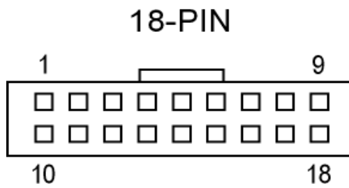
18-pin I/O connector (Looking at the acceptor)
